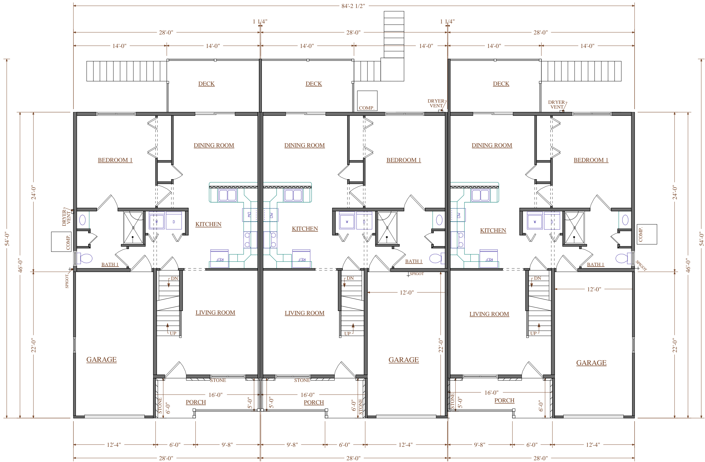
UNIT 2 FIRST FLOOR AREA 928.00 sq. feet
